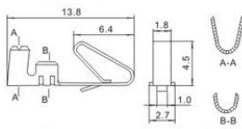
HX39602-PB (2139/3.96)
