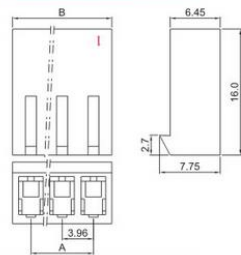
HX39603-NA (5271/3.96)
