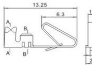
HX39602-Y (2139/3.96)
