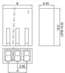
孔座 HOUSING(2139/3.96)
